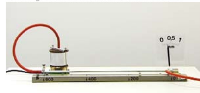
Dilatometer (3.1.2-1)
